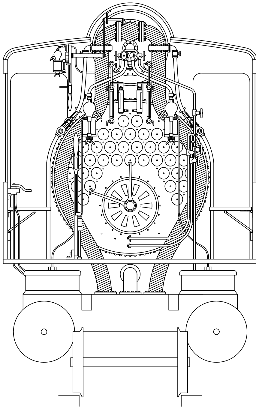
BACKHEAD DETAIL
