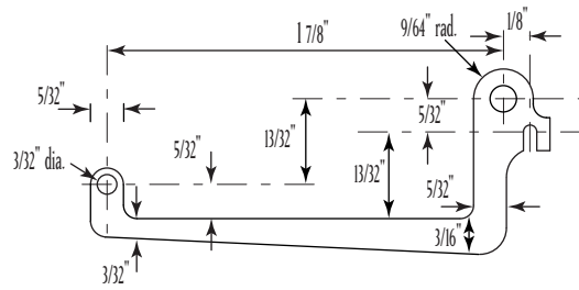
Coupling Matl. 10swg Mild Steel (2)
